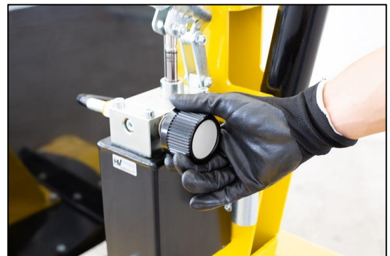
Detail of the hand pump with rod housing support and knurled knob
